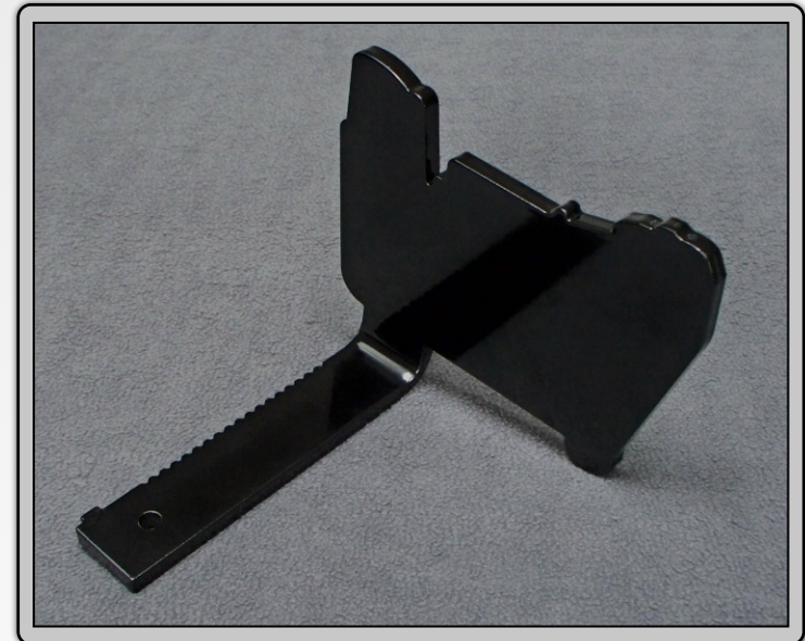
Laser-cut profile matches contours of both Ford -and- GM cases
